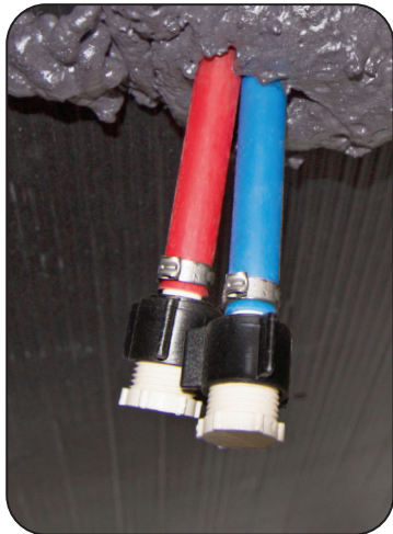
Low-Point Drain Valves located under the RV
