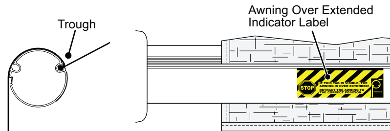
Awning Over Extended
